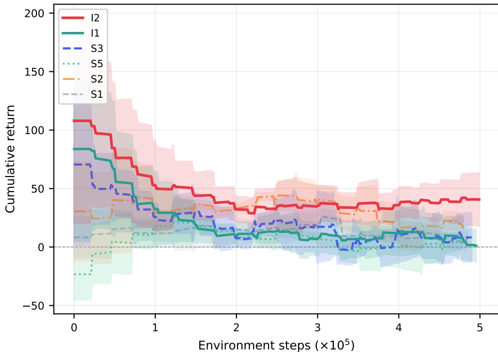
Test return — circular layout (mean \pm std)
